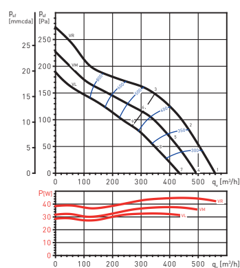
TD EVO 160
