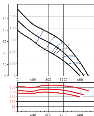
TD EVO 125
