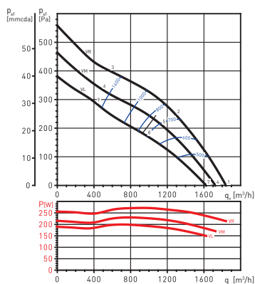
TD EVO 315
