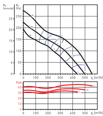
TD EVO 150
