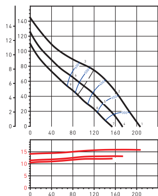
TD EVO 100
